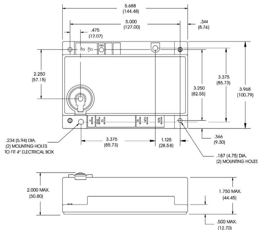
Figure 3. Standard Enclosure
