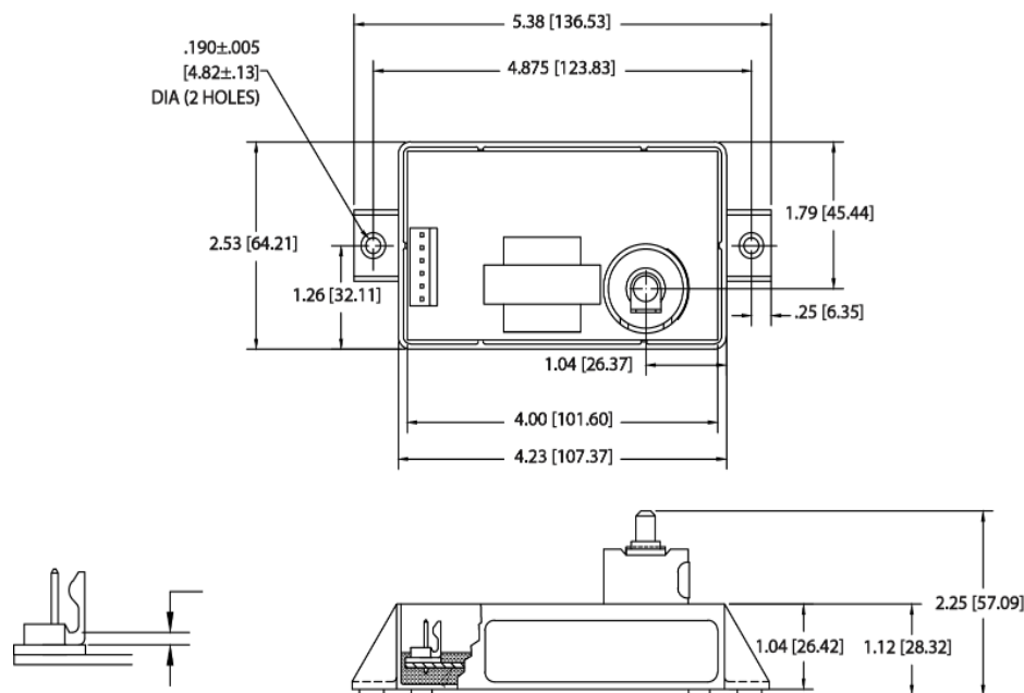
Figure 4. 35-602 Special Small Footprint Configuration
