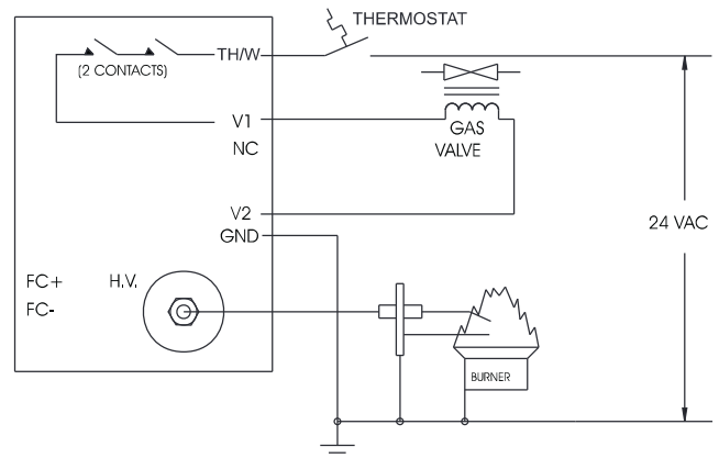
Figure 1. Local Sense
