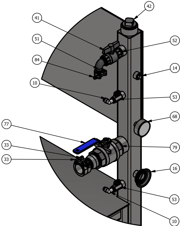
DETAIL G SCALE 1/8
