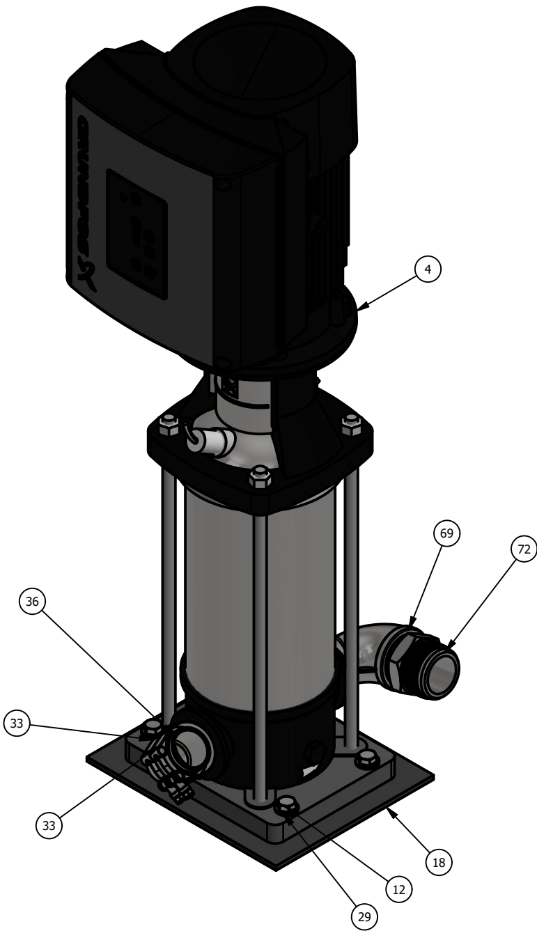
ISO ISOLATED VIEW SCALE 1/6
