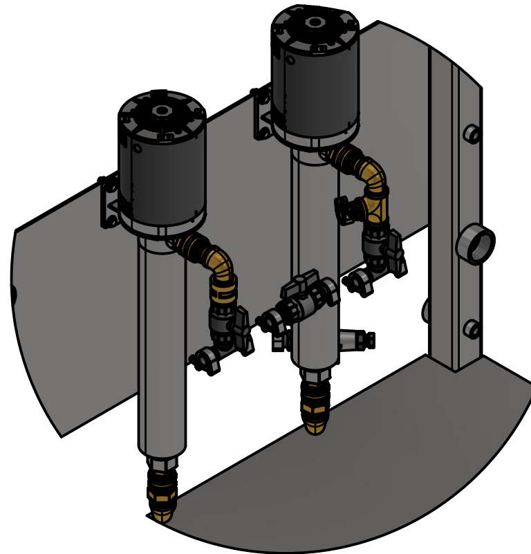
DETAIL B SCALE 1 /10
