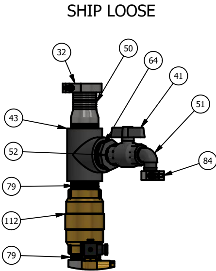
DETAIL F SCALE 1/8
